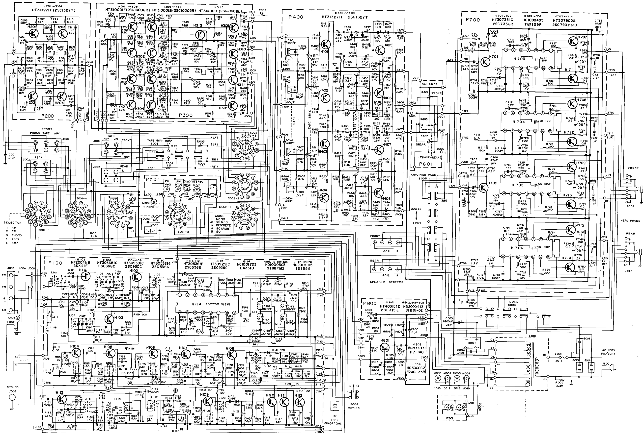
Figure 14. Schematic Diagram
